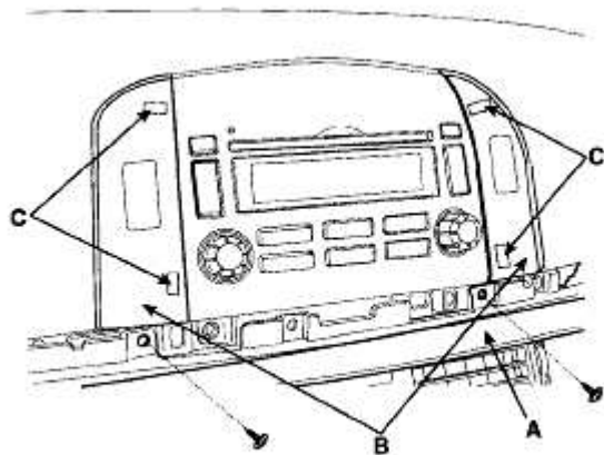
Fig. 10: Identifying Crash Pad Garnish, Center Facia Panel And Clips Courtesy of HYUNDAI MOTOR CO.
