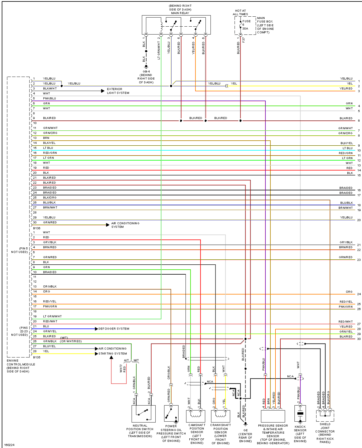
Fig. 8: Wiring Diagram (Impreza 2.5L & Outback Sport 2.5L - 1 Of 3)
